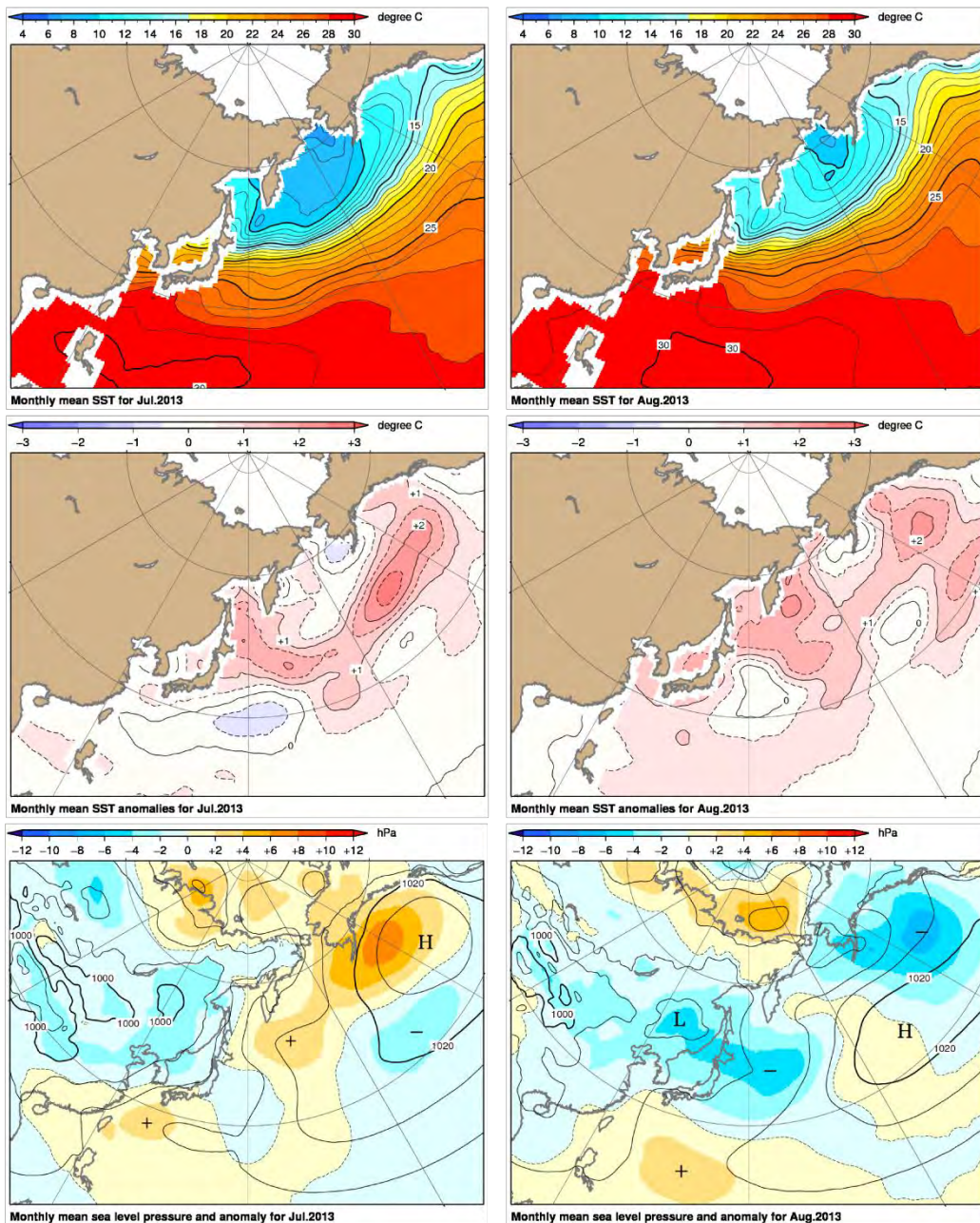
Fig. 1 Monthly mean sea surface temperature (upper), SST anomalies (middle) and sea level pressure (SLP) anomalies (bottom) for July and August 2013. Monthly mean SSTs and SLPs are based on JMA's COBE-SST (Centennial in situ Observation-Based Estimates of variability of SST and marine meteorological variables) and JRA-55 (Japanese 55-year Reanalysis), respectively. Anomalies are deviations from 1981–2010 climatology.
