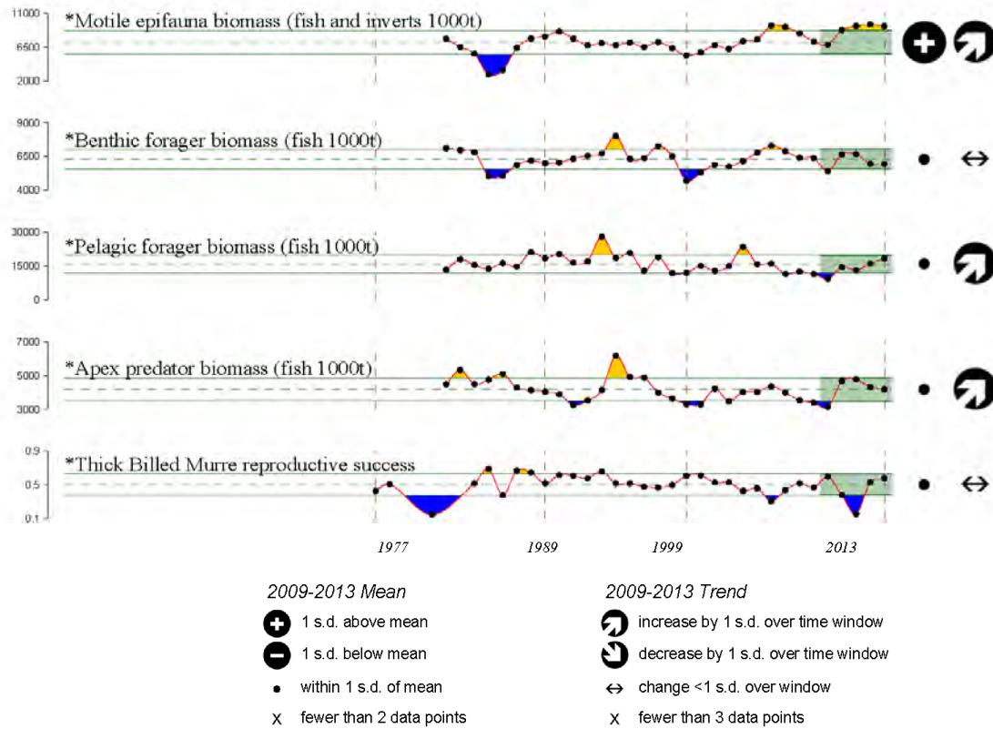
Fig. 3 Eastern Bering Sea ecosystem assessment indicators. * indicates time series updated in 2013.
