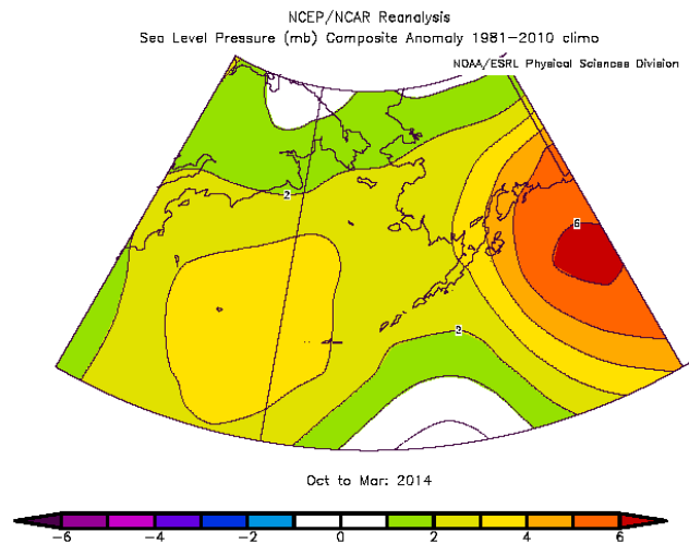
Fig. 1 NOAA sea level pressure (mb) composite anomaly (deviations from 1981–2010 climatology) for October 2013–March 2014. Figure courtesy of N. Bond.
