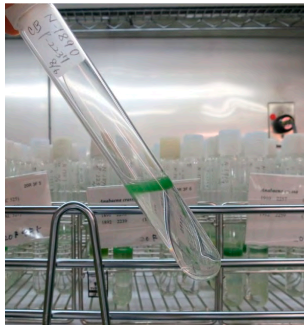
Test tube of Anabaena .
