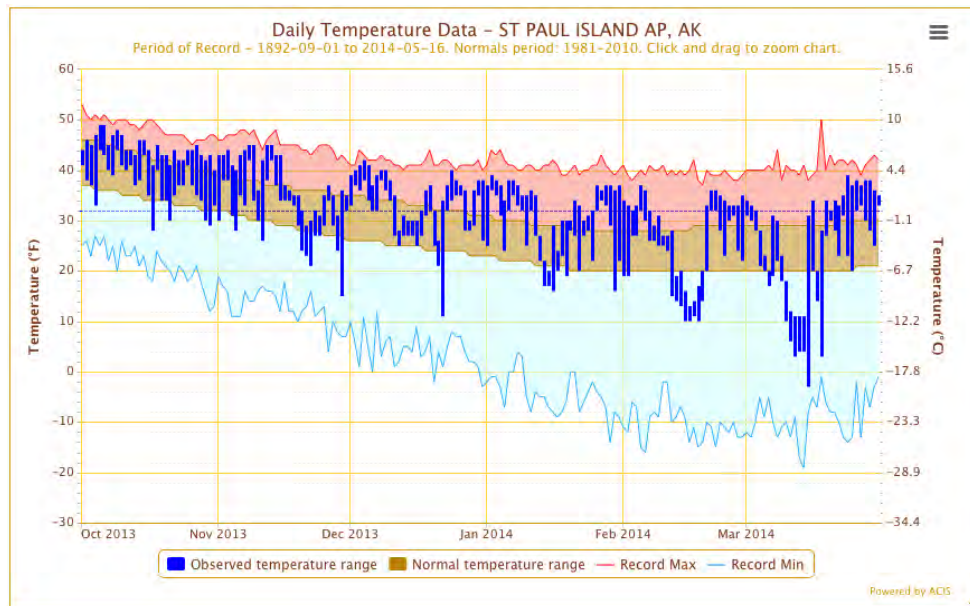
Fig. 2 Daily air temperature (°F) at St. Paul Island October 2013–March 2014. The reddish and aqua lines at the top and bottom, respectively, refer to the all time high and low temperatures for each date; the tan lines in the center refer to the average daily high and low temperatures for each date. The period of record is 1892 to present. Figure courtesy of N. Bond.
