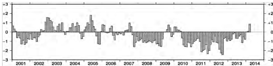
Fig.3 Time series of Pacific Decadal Oscillation (PDO) index from January 2001 to March 2014.
