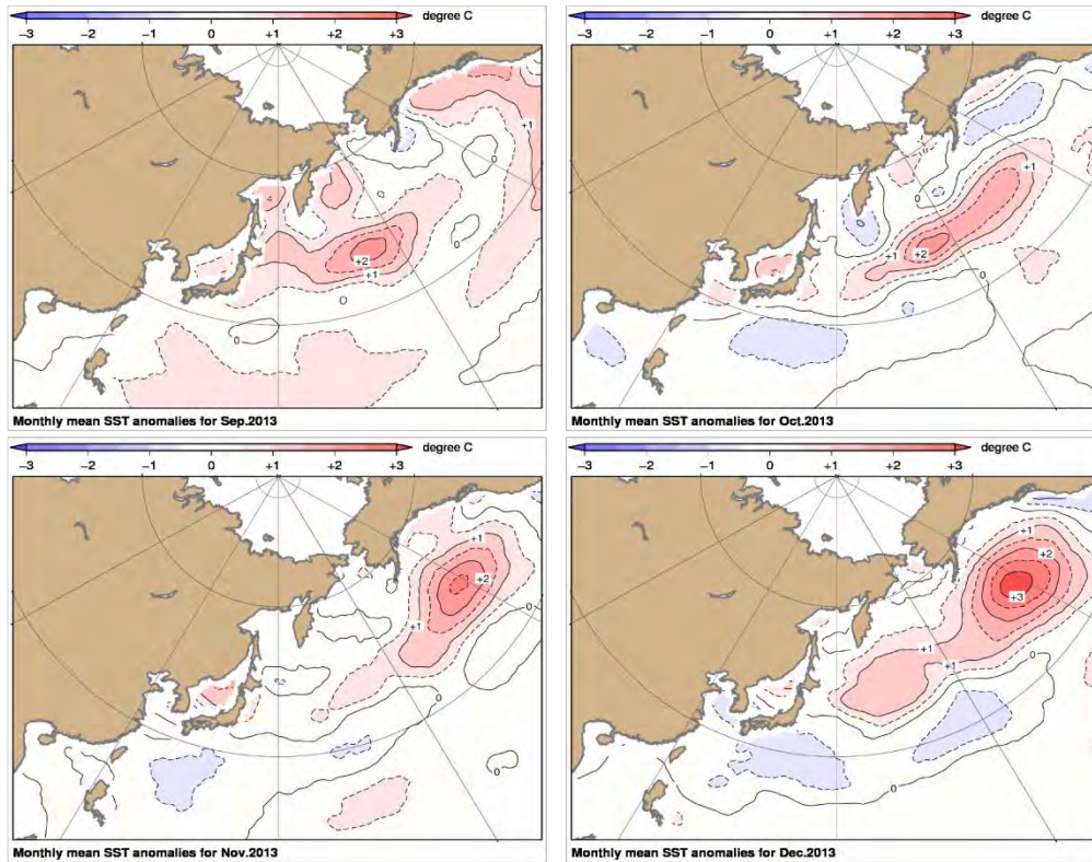
Fig.2 Monthly mean SST anomalies from September to December 2013.
